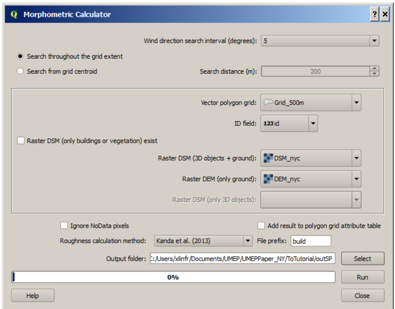
Fig. 9.17: The settings for calculating building morphology.
