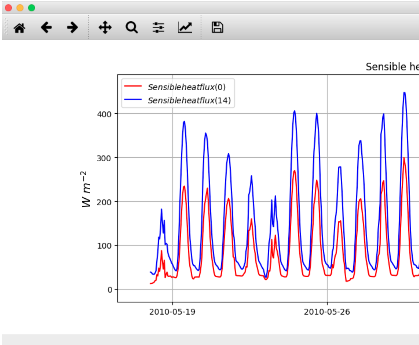
Fig. 9.26: Example of the comparison of the heat flux for two grid cell in the vector grid.
