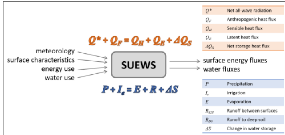
Fig. 1.1: Overview of SUEWS
